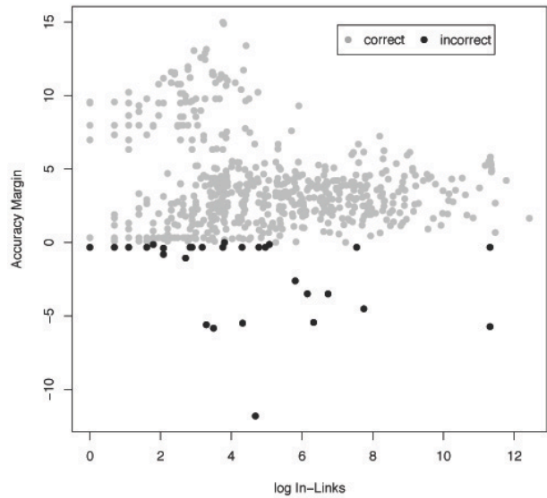
Figure 2. log(In-Links) vs. Accuracy(URL)
